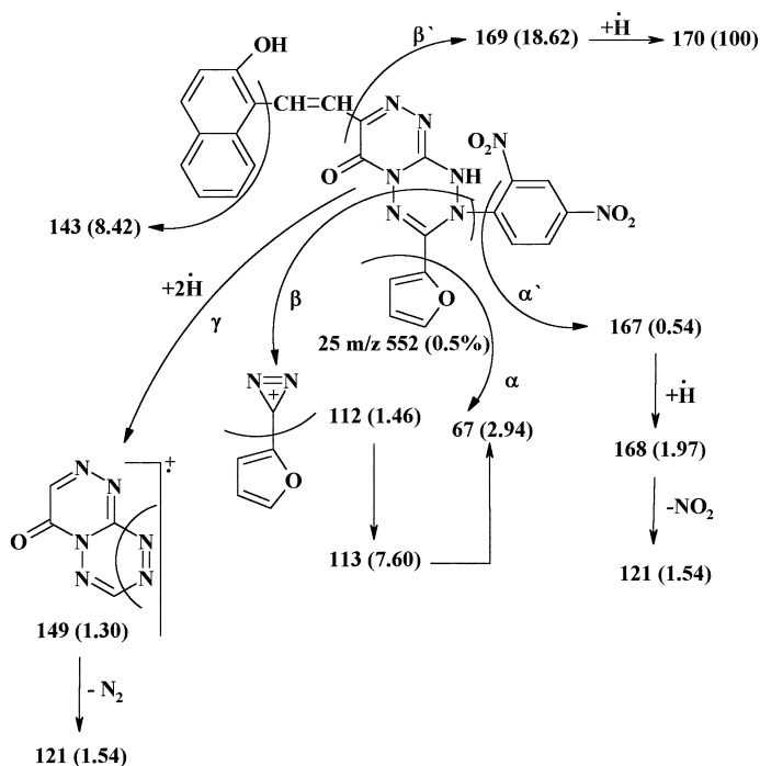
FIGURE 2 Mass fragmentation of compound 25 .
