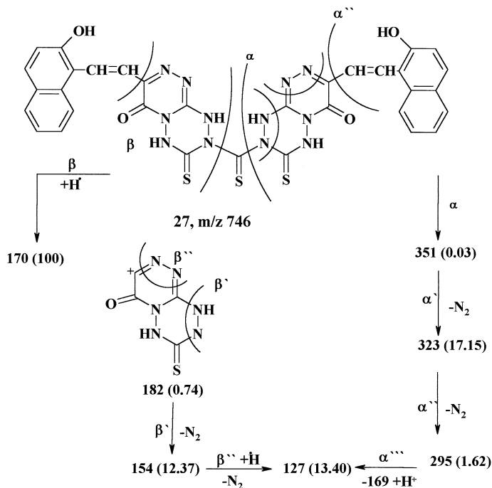
FIGURE 3 Mass fragmentation of compound 27 .
