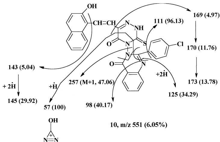
FIGURE 1 Mass fragmentation of compound 10 .
